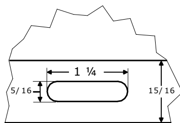
Mounting Holes (x10) DETAIL A
