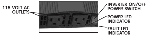
Figure 1 Front Panel
